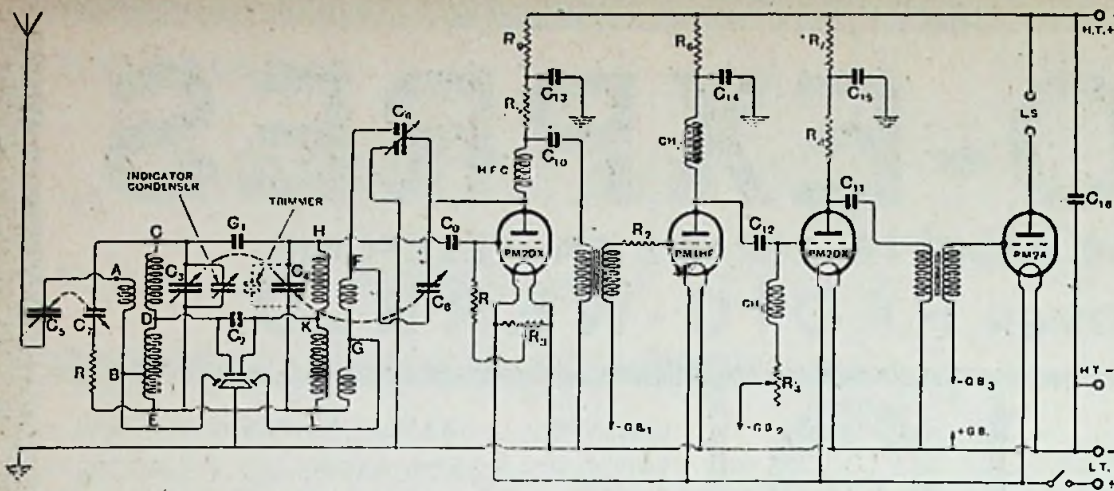
Principeschema van de Wireless World Autotone. C_1 2.5 \mu\mu\text{F} ; C_2 2.0 \mu\mu\text{F} ; C_3, C_4 500 \mu\mu\text{F} ; C_5 300 \mu\mu\text{F} ; C_6 300 \mu\mu\text{F} (diff.); C_7, C_8 30 \mu\mu\text{F} ; C_9 100 \mu\mu\text{F} ; C_{10}, C_{11} 1 \mu\text{F} ; C_{12} 4 \mu\text{F} ; C_{13}, C_{14}, C_{15}, C_{16} 2 \mu\text{F} ; R 30 \Omega ; R_1 0.25 M \Omega ; R_2 50000 \Omega ; R_3 400 \Omega ; R_4 5000 \Omega ; R_5, R_6, R_7, R_8 30000 \Omega ; R_9 50000 \Omega ; CH_1 0.3 H; CH_2 ong. 30 Henry.
